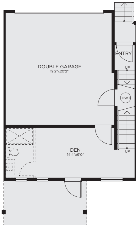
LOWER FLOOR 306 SQ FT
