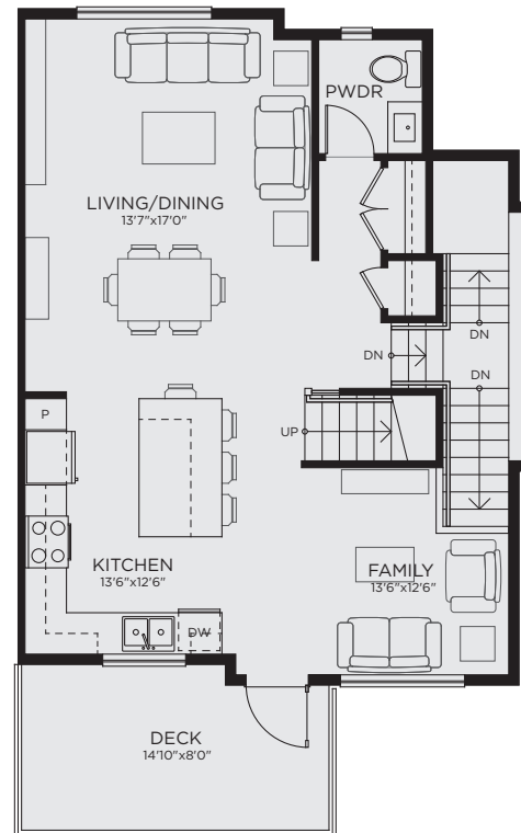
MAIN FLOOR 757 SQ FT
