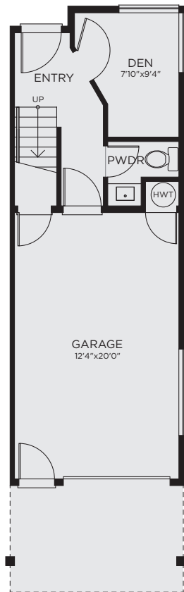
LOWER FLOOR 198 SQ FT
